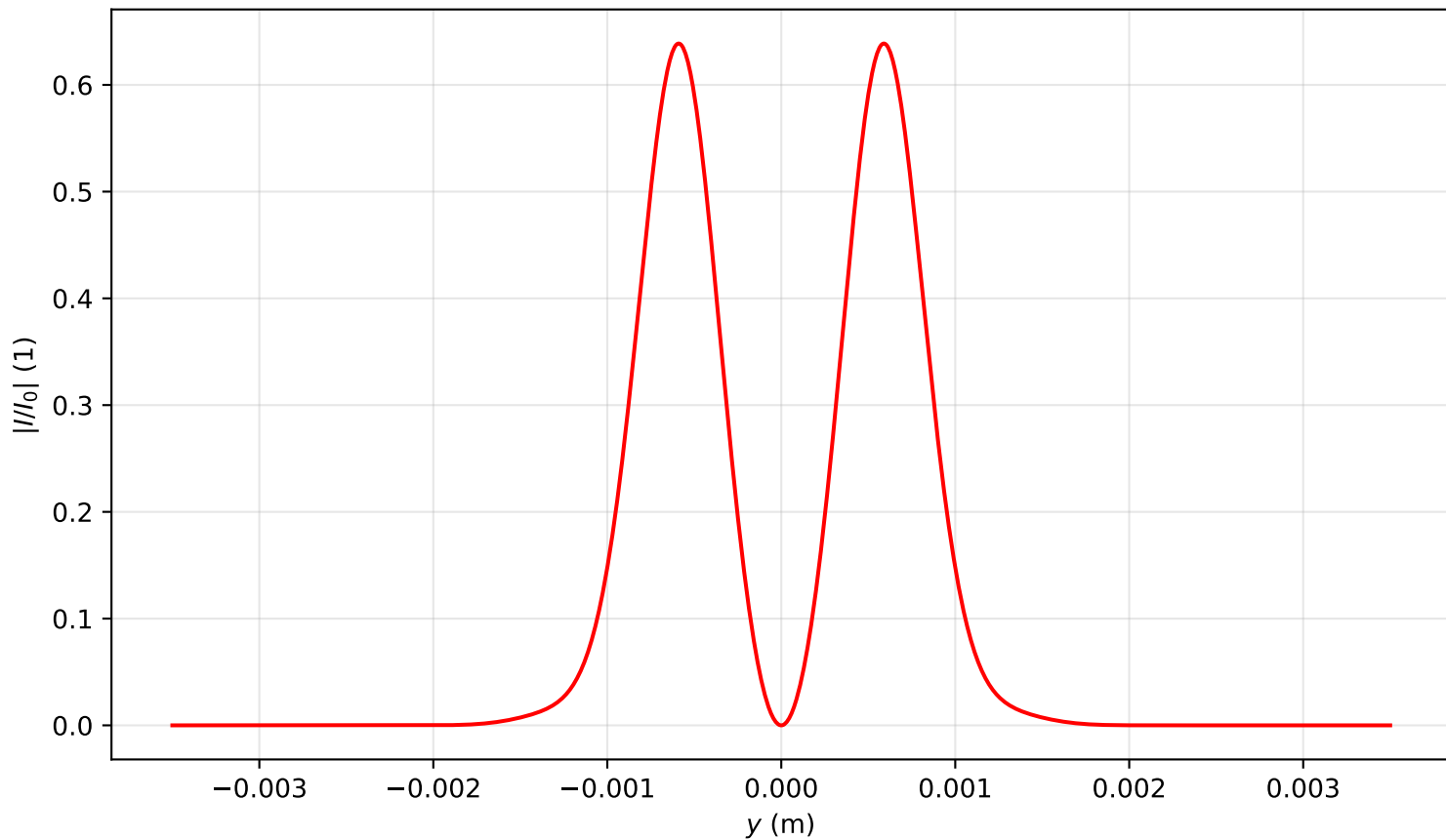
Intensity profile I(x=0, y, z=1.035)/I_0 , P_{in}=2.0P_{cr} , artificial time
